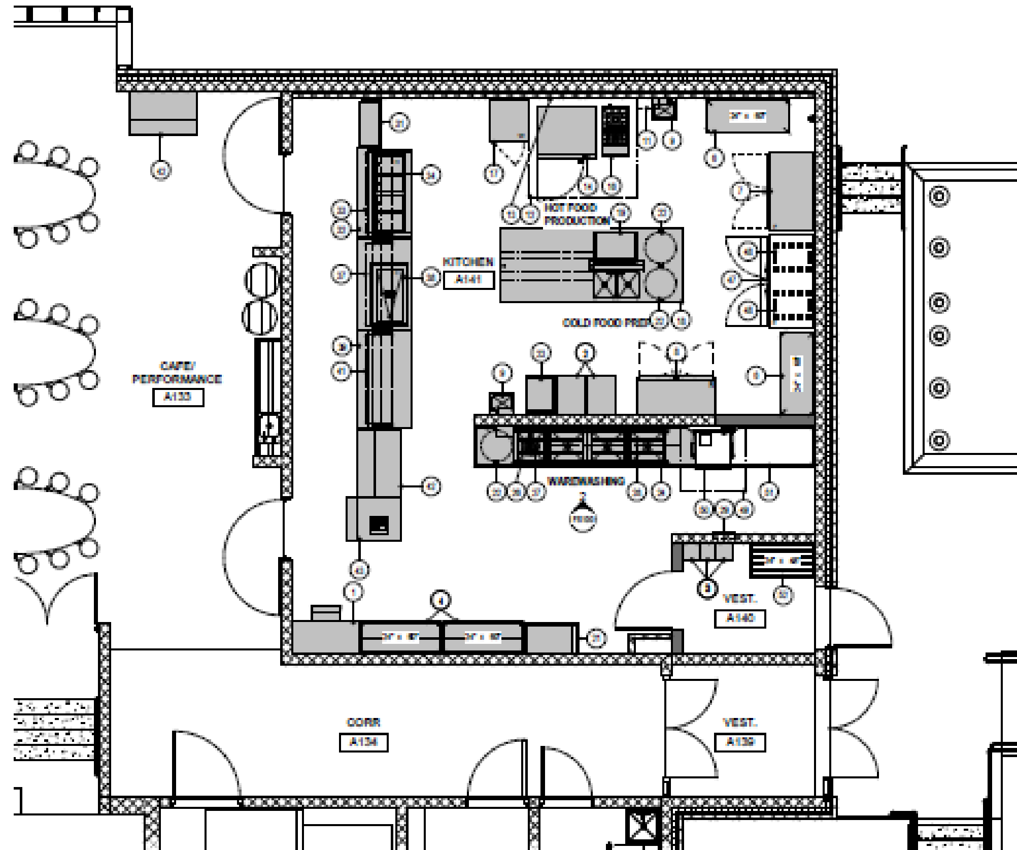
1 FOODSERVICE EQUIPMENT PLAN 1/4" = 1'-0"
